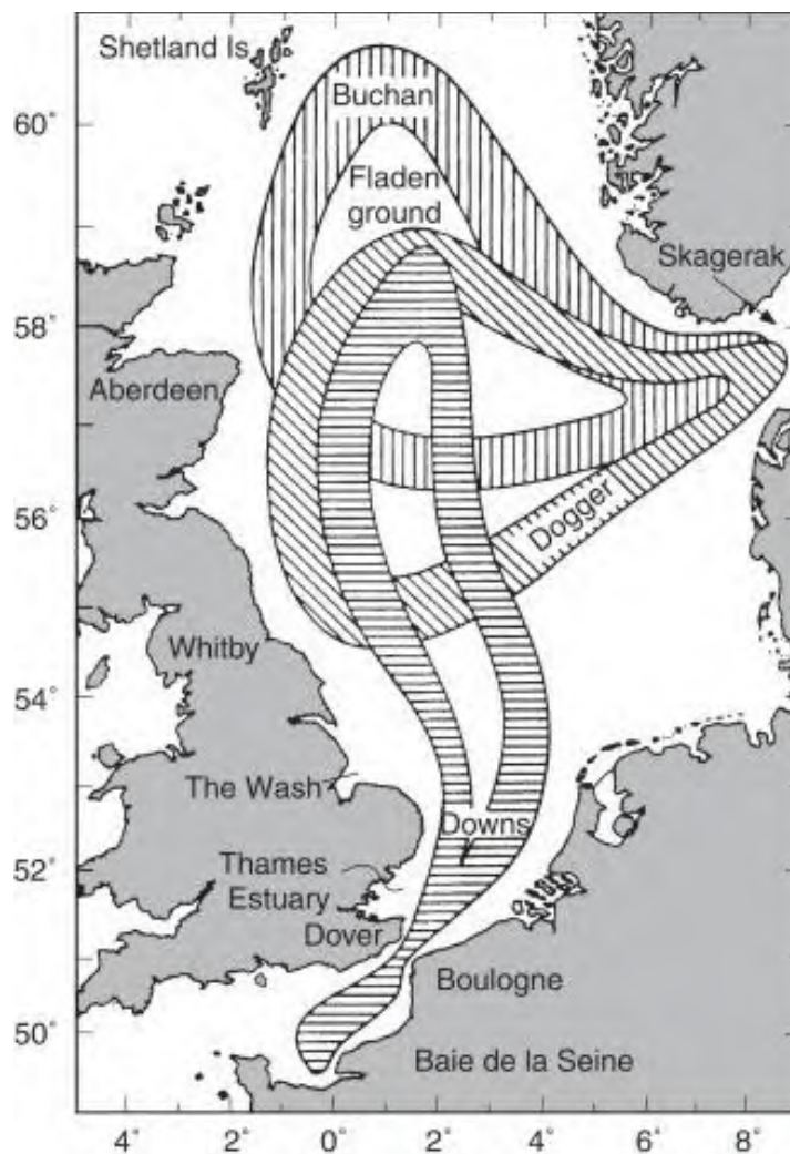
Plate 10.1: The migration circuits of the three groups of spawners in the North Sea: Buchan, Dogger and Downs (taken from Cushing, 2001).
